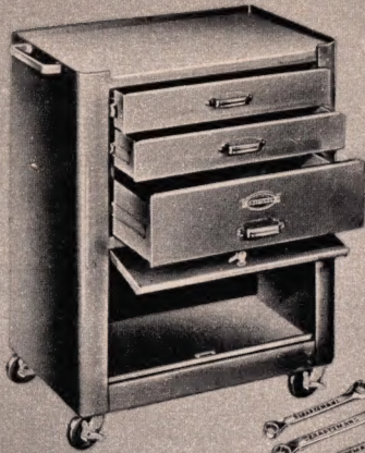
CRAFTSMAN Roller Cabinet included, 17 in. deep; 25½ in. wide; 32 in. high. See 99 C M4358, page 27.
